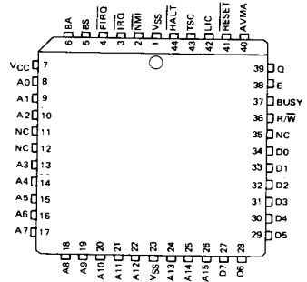
FN SUFFIX PLCC 44
